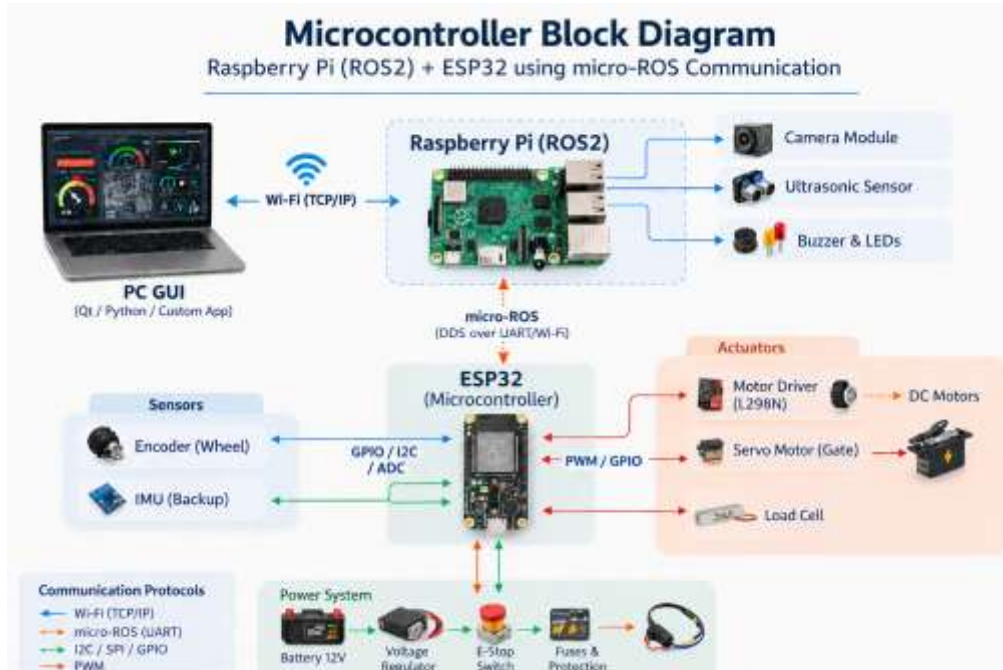
Figure 1— System block diagram: Raspberry Pi (ROS 2) + ESP32 over micro-ROS, with sensors, actuators, power chain and communication protocols.
