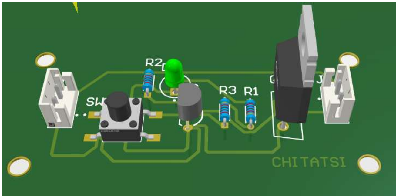
Figure 5 Safety Circuit
