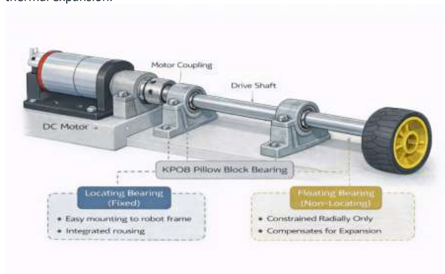
Figure 3 Bearing Placement Configuration
